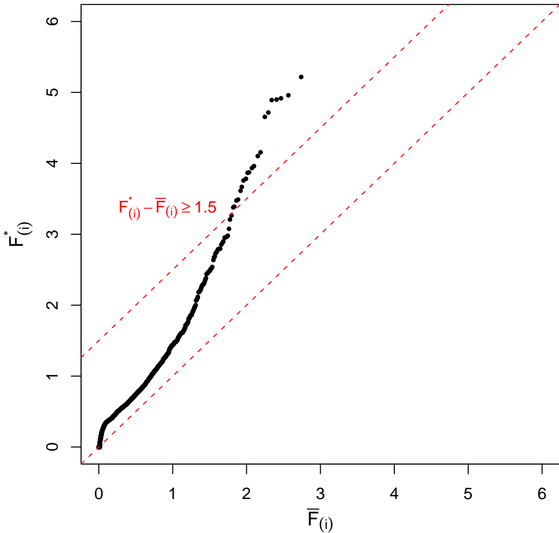
Penalized-F with \lambda = 37.63
