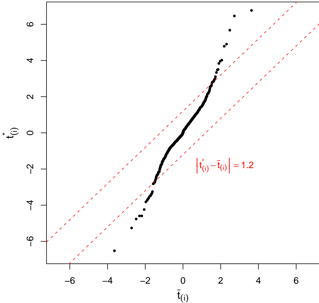
Penalized-T with \lambda = 21.74
