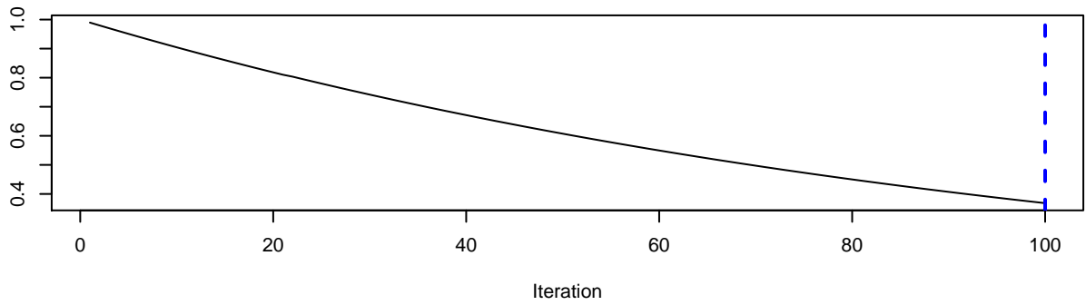
AdaBoost exponential bound
